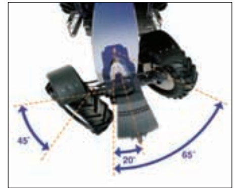
The SuperSteer axle moves the inside wheel out and away from the tractor frame, providing more tire clearance and a greater turn angle for faster, sharper turns. Add the 20 degrees of axle articulation to the standard turn angle of 45 degrees for an unmatched total turn angle of 65 degrees.
